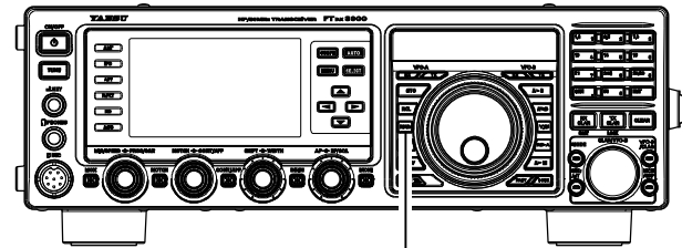
[NAR] Button
