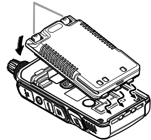
Battery latches
